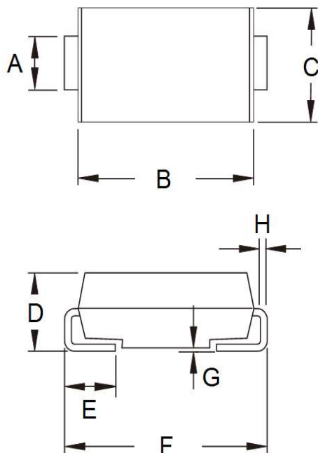
DO-214AA (SMB)
